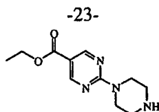
intermediate 2
